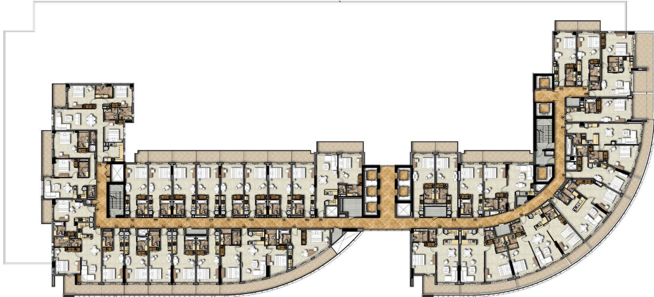
TYPICAL FLOOR PLAN Level 16
